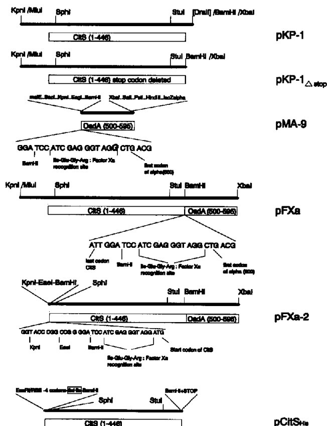
Fig. 1. Schematic representation of plasmids encoding CitS (pKP-1, pKP-1 \Delta stop), CitS \alpha (pFXa, pFXa-2), CitS His (pCitS His ) and the MalE- \alpha (500–595) fusion (pMA-9). Only the inserts and the vector parts used in the construction are shown. The deleted base ('G') in pMA-9 is shown in bolder letter-type (for details see text).
